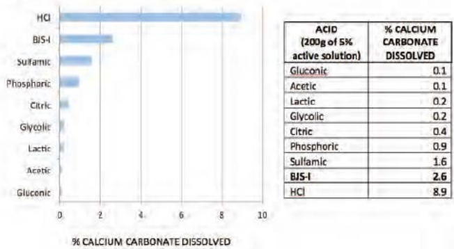
CALCIUM CARBONATE DISSOLVING PROPERTIES OF ACIDS: 3 MINUTE EXPOSURE (SURFACE SCALE REMOVAL)
